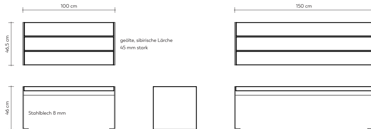
Bank klein
